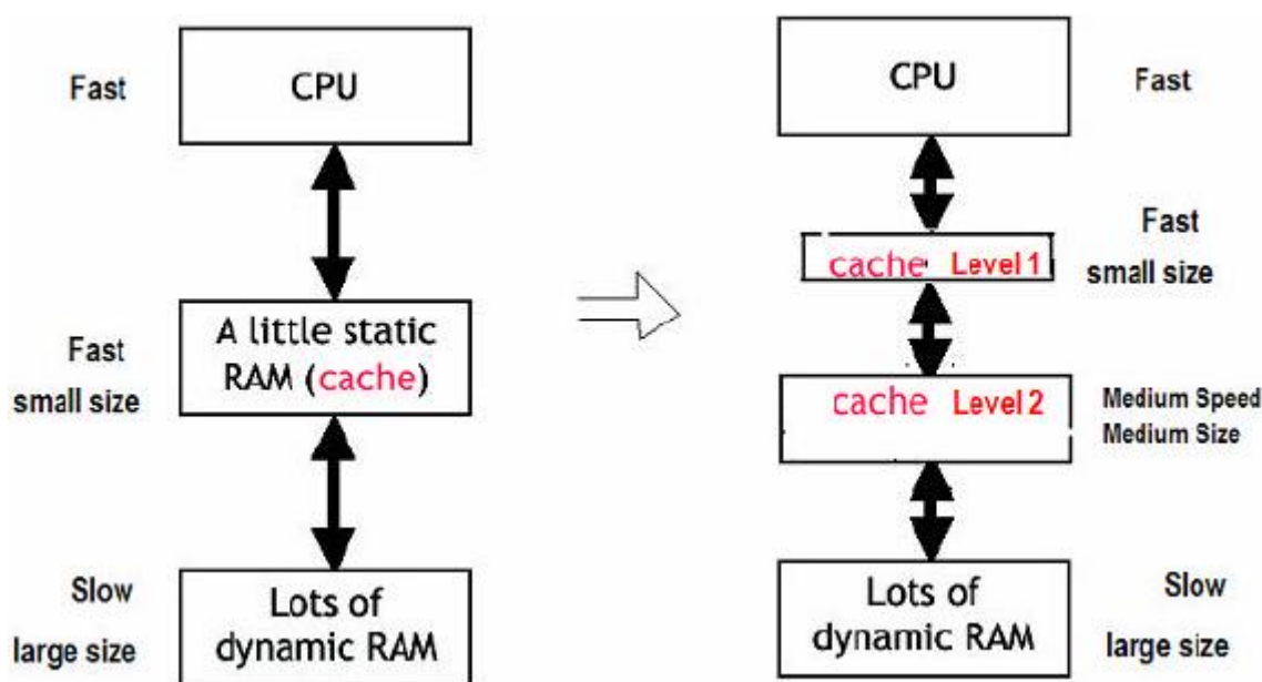
Figure 1. Concept of a multilevel cache
