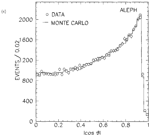
Fig. 7a-c. Distributions for events with the track-based selection. a) Total charged energy divided by the beam energy. b) Multiplicity of charged tracks. c) Absolute value of the cosine of the angle of the sphericity axis with respect to the beam direction
