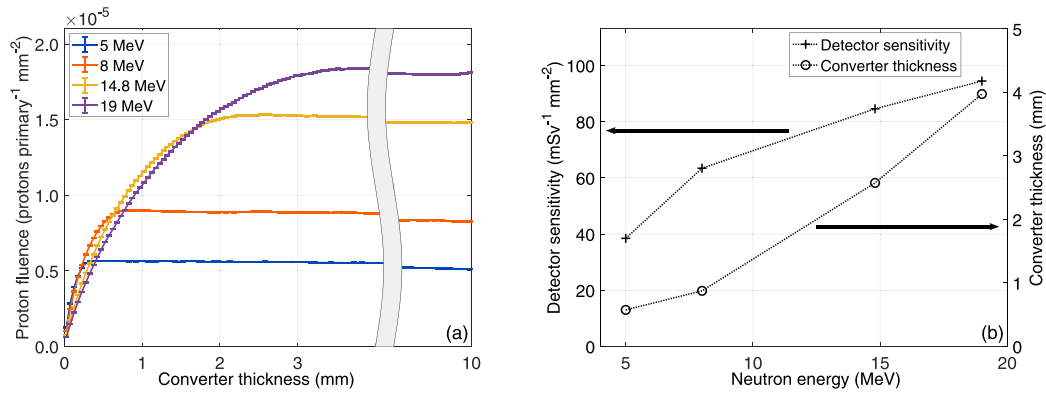
Fig. 5. Monte Carlo study of the optimisation of converter thickness for higher neutron energies. (a) Proton fluence as a function of converter thickness. (b) Maximal detector sensitivity at 2\mu\text{m} depth of the FNTD and corresponding converter thickness. As the uncertainties are smaller than the marker size, the error bars are not displayed. In both plots, the dots are connected with lines for visual aid.
