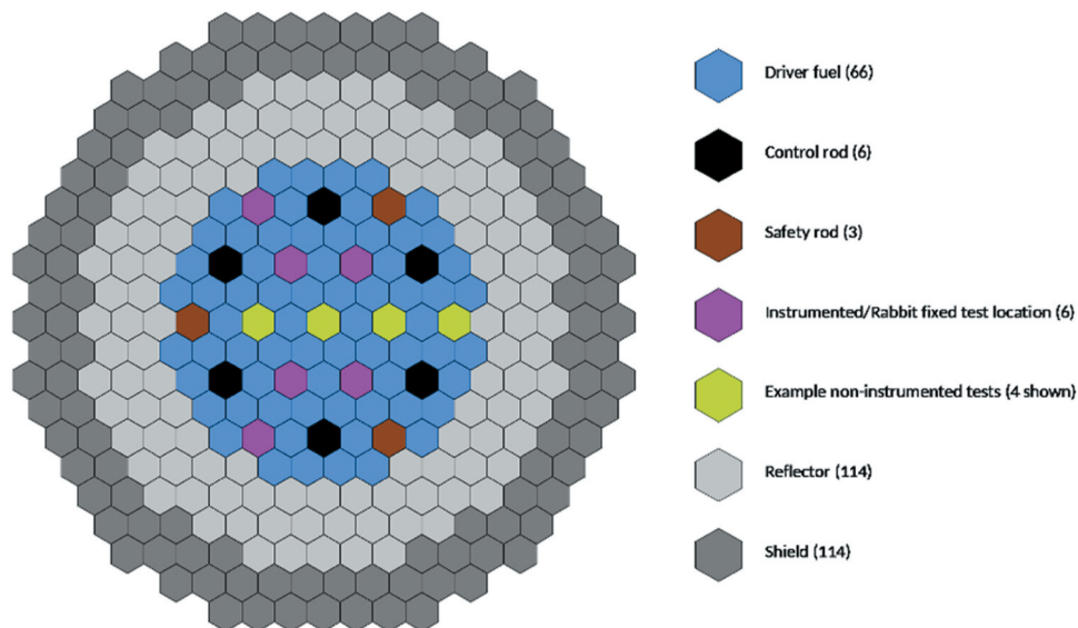
Fig. 1. VTR core radial layout.
