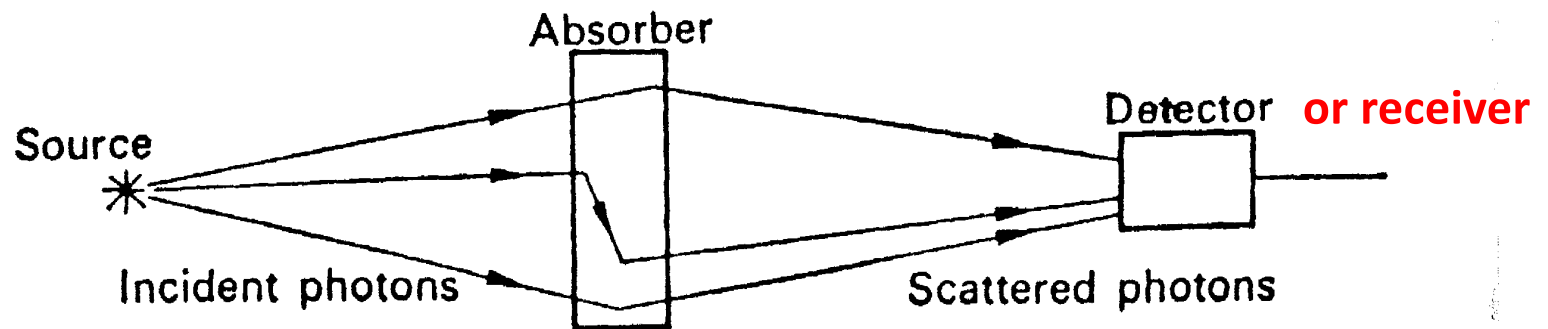
FIGURE 10.5. Gamma-ray absorption under conditions of broad beam geometry, showing the effect of photons scattered into the detector.
