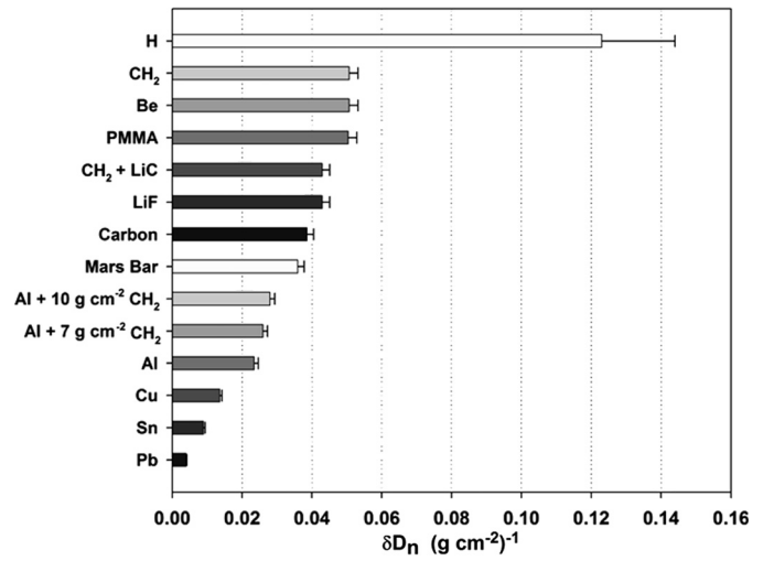
Fig. 5. Dose attenuation properties of a variety of shielding materials exposed to 1 GeV/n 56 Fe-ions. Bragg curves were measured by the LBL group at the Brookhaven National Laboratory. \delta D represents the initial slope of the Bragg curve (Eq. (5)), extrapolated to zero-thickness. Plot modified from Zeitlin et al. (2006), courtesy of Cary Zeitlin.
