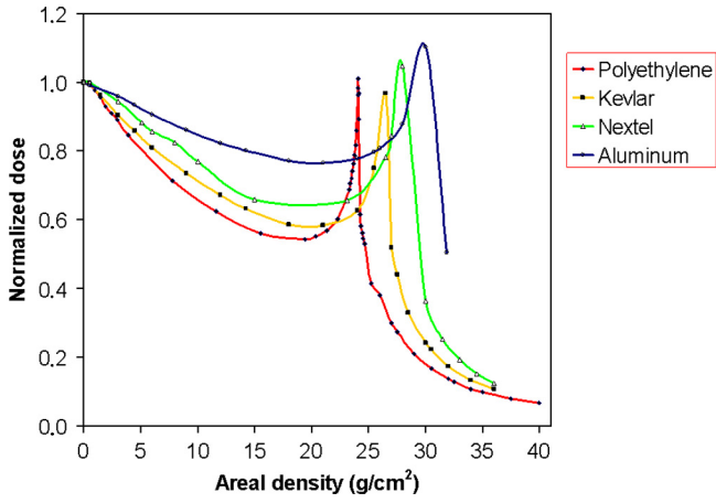
Fig. 4. Measured Bragg curve of 1 GeV/n Fe ions in polyethylene, aluminum, Kevlar, and Nextel. The normalized dose is plotted vs. the thickness in g/cm 2 . Materials effective for GCR shielding have a higher initial slope \delta D and shorter range. Polyethylene is clearly better than Al, and Kevlar is close to polyethylene. Measurements at the Brookhaven National Laboratory (Upton, NY), figure modified from Lobascio et al. (2008).
