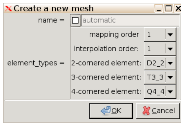
Figure 28: New mesh
