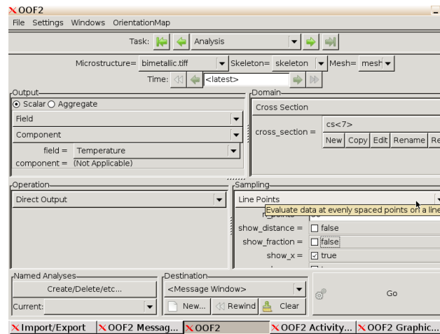
Figure 45: Analysis pane
