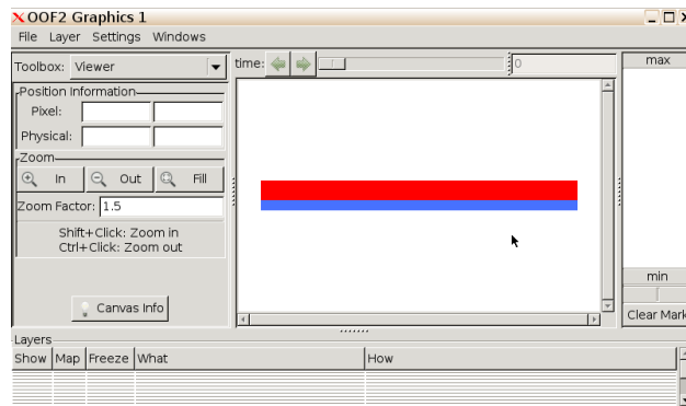
Figure 5: Graphics window
