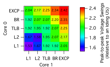
Fig. 13: Impact of microarchitectural event interference across cores.
