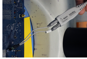
(b) Sensing voltage using an InfiniiMax 1.5GHz 1130A differential probe that has ultra low loading.
