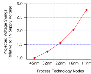
Fig. 1: Voltage noise is increasing in future generations.
