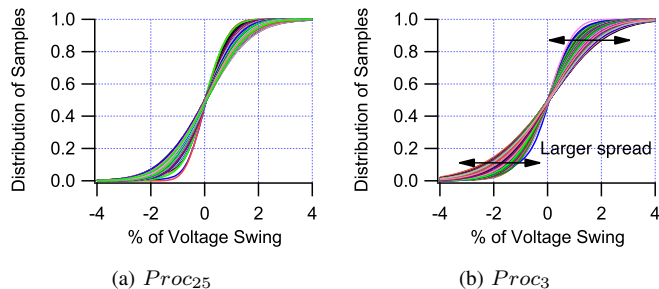
Fig. 9: Typical-case swings in future processors are increasingly more slanted compared to Proc_{100} (see Fig. 7) as voltage noise grows.
