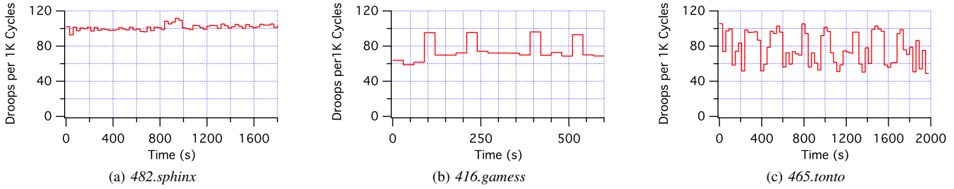
Fig. 14: Single-core droop activity until complete execution. Some programs show no phases (e.g., 482.sphinx ). Others, like 416.gamess and 465.tonto , experience simple, as well as more complex phases, respectively.
