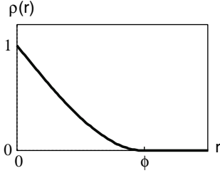
Figure 1. Spherical function.
