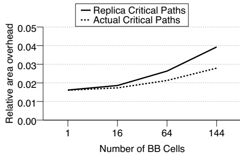
Figure 21. Area overhead of D-FGBB as a fraction of the chip area.
