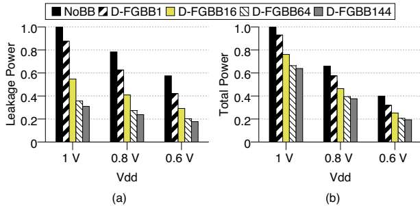
Figure 20. Leakage (a) and total power (b) at different voltage-frequency pairs, without and with D-FGBB.
