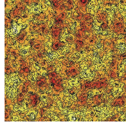
Figure 3. Systematic V_{th} variation map for a chip with \phi = 0.1 .
