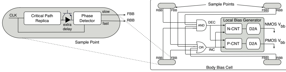
Figure 6. Proposed circuit to support D-FGBB in a cell.
