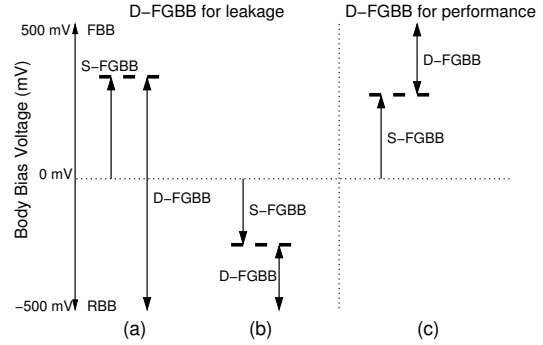
Figure 8. Changing the BB voltage with D-FGBB.
