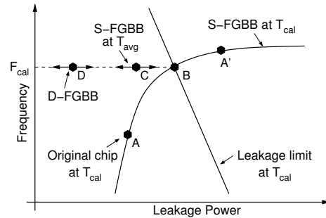
Figure 12. Impact of S-FGBB and D-FGBB on a chip’s operating point.
