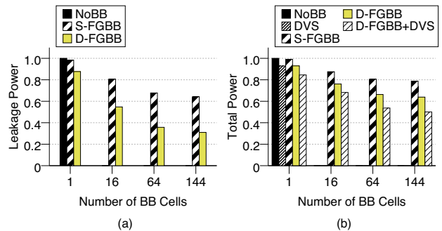
Figure 19. Leakage (a) and total power (b) of the chips for different FGBB schemes at constant frequency.
