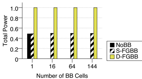
Figure 18. Total power of the chips for different FGBB schemes.
