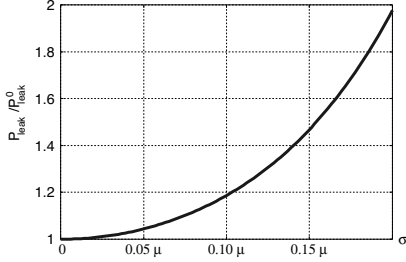
Figure 4. Relative leakage power in the chip as a function of V_{th} 's \sigma .
