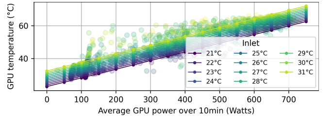
Figure 7. GPU temperature as a function of inlet temperature and GPU power load over 10 minutes using data from Figure 6 . The figure includes a regression curve based on inlet temperature and GPU load.
