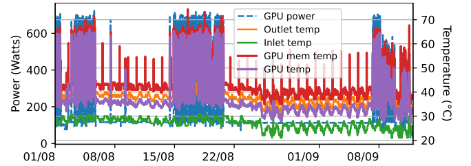
Figure 6. GPU and memory temperature over time alongside inlet temperature.
