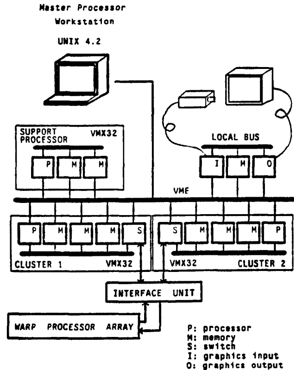
Figure 6-1: Host of the Warp machine
