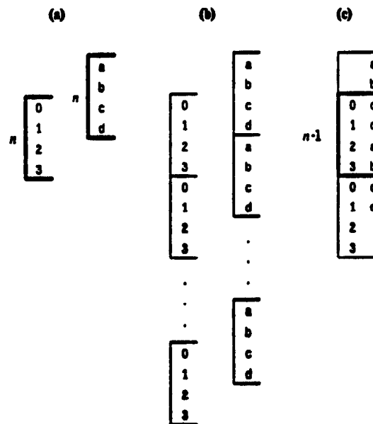
Figure 4-2: Merging two iterative processes (a) original programs (b) execution trace, and (c) merged programs
