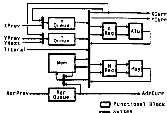
Figure 2-2: Warp cell data path
