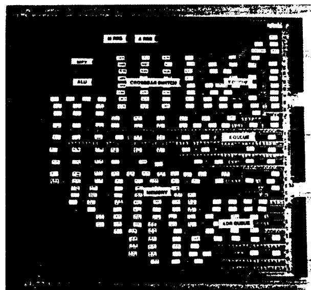
Figure 2-3: Warp cell layout
