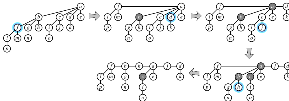
Decreasing the keys of four nodes: first f, then d, then j, and finally h. Dark nodes are marked. DECREASEKEY(h) causes nodes b and a to be recursively promoted.
