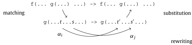
Fig. 6. Behavior of amatchrew.
