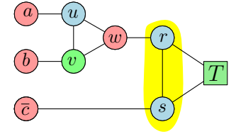
Figure 38.5: The formula (a \vee b \vee c) \wedge (b \vee \bar{c} \vee \bar{d}) \wedge (\bar{a} \vee c \vee d) \wedge (a \vee \bar{b} \vee \bar{d}) reduces to the depicted graph.
