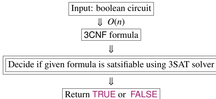
Figure 37.5: Reduction from CSAT to 3SAT
