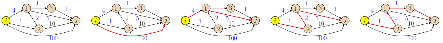
Figure 5.10: The intermediate shortest paths: \text{dist}(i, j, 0) = 100 , \text{dist}(i, j, 1) = 9 , \text{dist}(i, j, 2) = 8 , \text{dist}(i, j, 3) = 5 .
