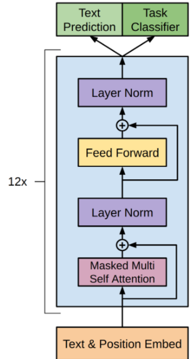
GPT-1 Model
