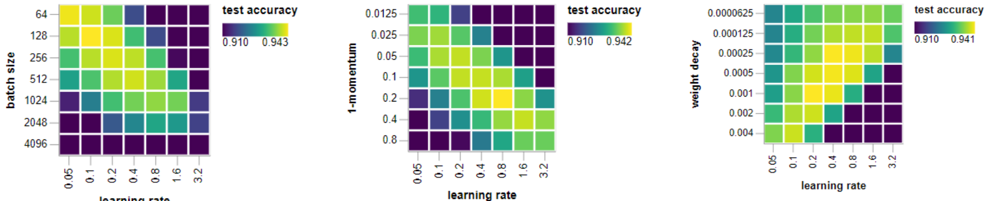
Fig: https://myrtle.ai/learn/how-to-train-your-resnet-5-hyperparameters/
