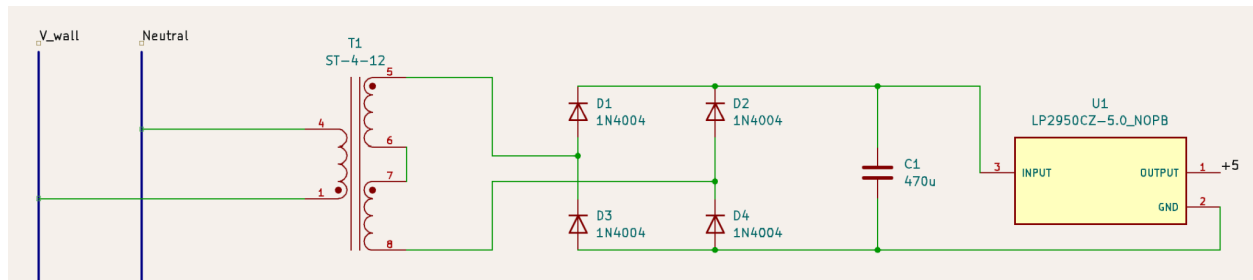
Figure 4: 5 V AC-DC converter
