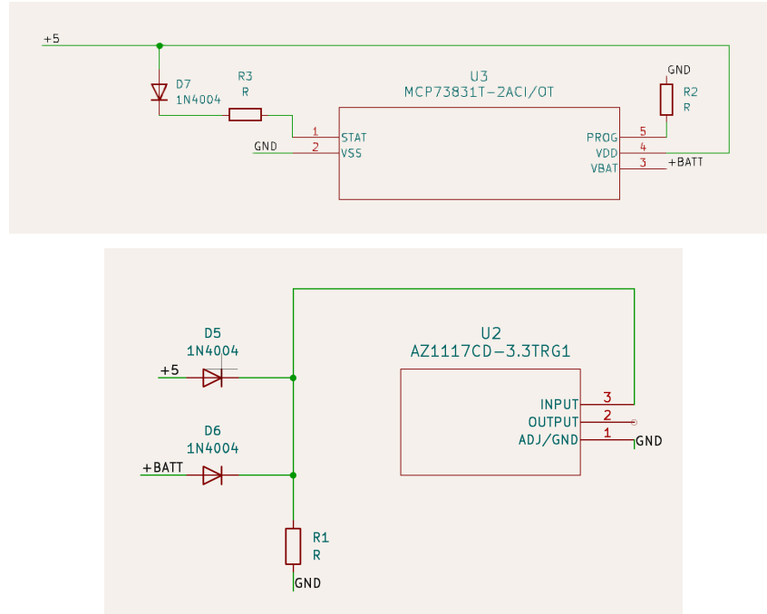
Figure 5: Battery charger circuit, OR circuit, 3.3 V regulator
